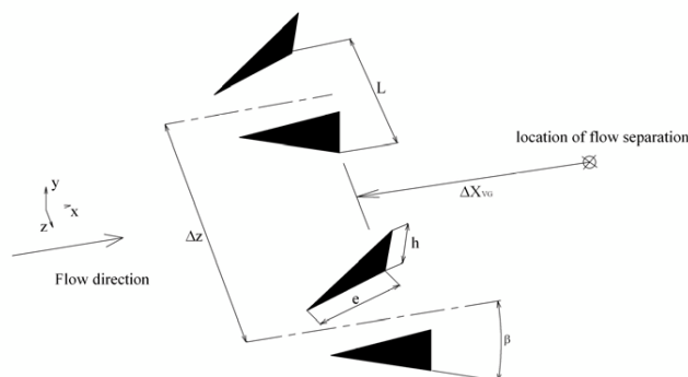
Figure: 2 VGs design and its relative position
