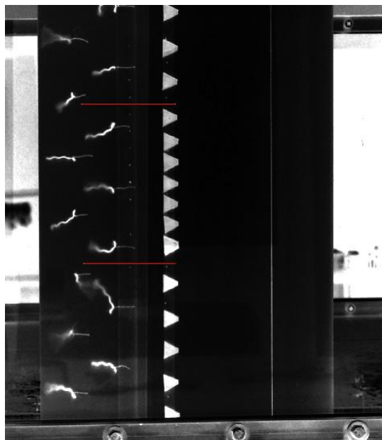
Figure: 4 Rectangular VG ( h=3\text{mm} , \Delta z=16\text{mm} , red lines area), 20 0
