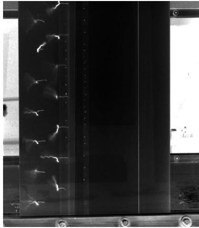
Figure: 3 Non-controlled case, 20 0 deflected flap, \alpha = 0^\circ
