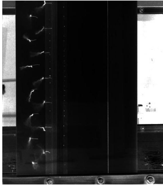
Figure: 5 Triangular VG (h=3mm, \Delta z=9\text{mm} ) 0^\circ deflected flap, \alpha = 0^\circ
